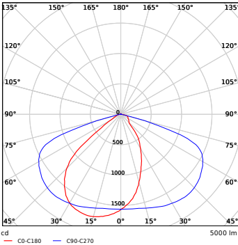
LEDStreetlight-E2 40W
