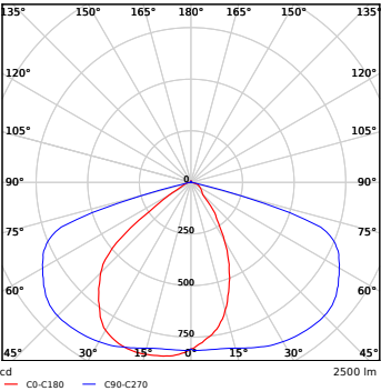
LEDStreetlight-E2 20W
