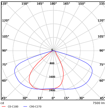
LEDStreetlight-E2 60W
